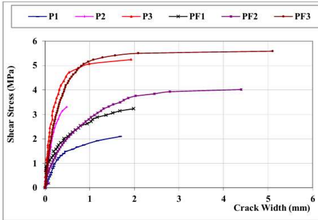
Fig. 2. Dependence " \tau - a " for the P and PF series
