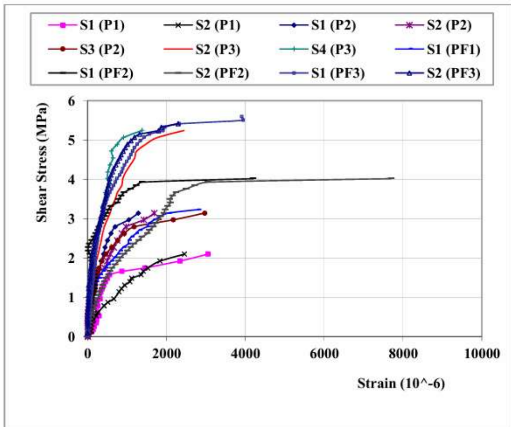
Fig. 3. Dependence " \tau - \varepsilon " in steel clamps across the cut plane of reinforced (P series) and non-reinforced (PF series) special samples
