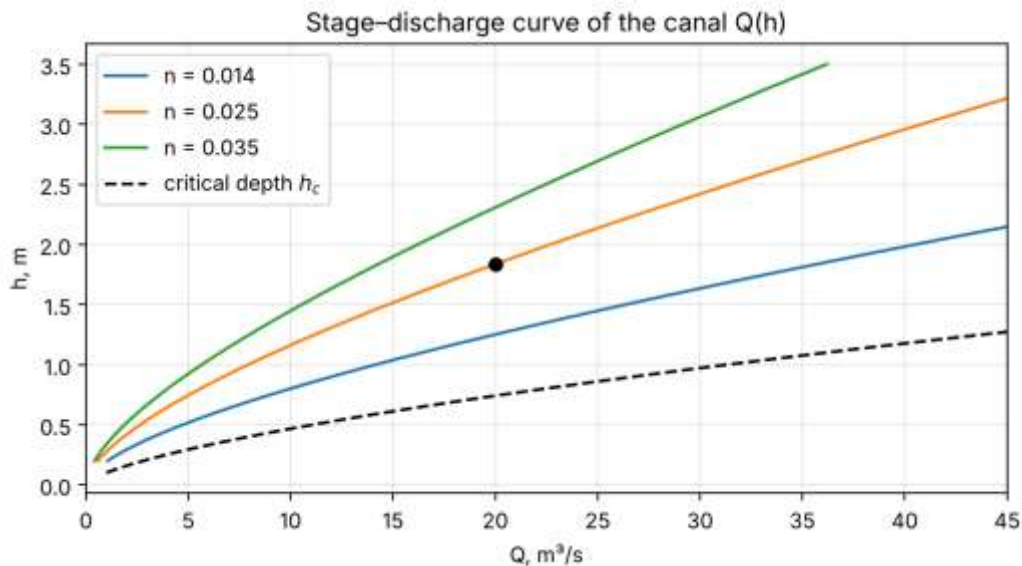
Figure 1. Stage–discharge curves Q(h) of the canal for different roughness coefficients; dashed line – critical depth, dot – worked example
